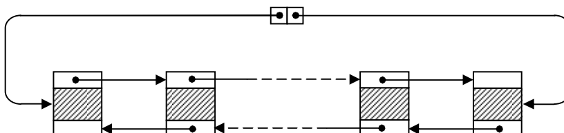
Fig. 4.56. Bidirectional list
